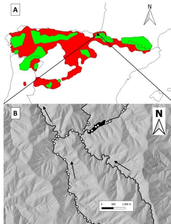
Figure 1. (A) Historical (in red) and current (in green) distribution of the Pyrenean Desman and location of the study site (black dot). (B) The stream network in Artikutza Valley with the location of artificial latrines (white dots). The black area represents the area formerly drowned by the Enobieta Reservoir, and the black arrows indicate the flow direction.
