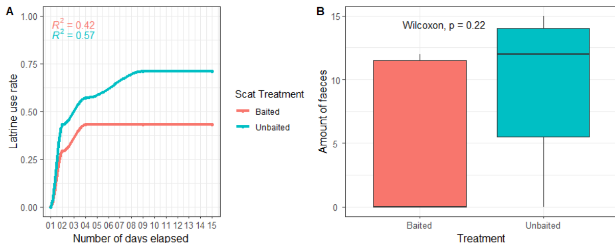
Figure 3. (A) LOESS models of the use rates of baited vs unbaited latrines from their installation (day 1) to the end of the experiment (day 15). (B) Amount of faeces found in baited vs unbaited latrines
